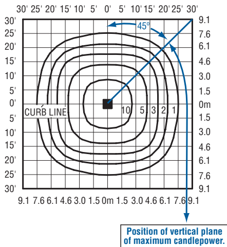
Isofootcandle plot of 6000K, 60 LED Type V Short 304 series canopy luminaire at 15' A.F.G. Luminaire with 11,409 initial delivered lumens operating at 700mA. Initial FC at grade.
