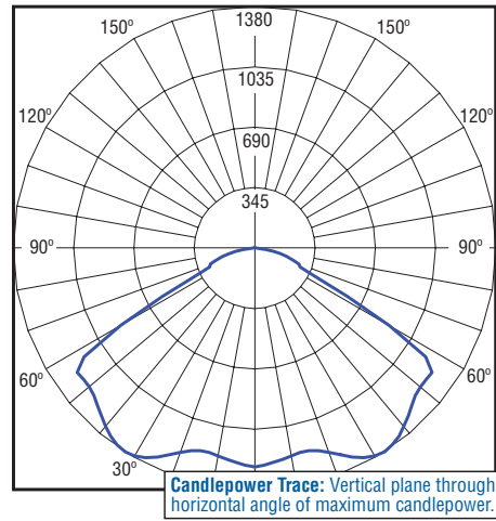
Independent Testing Laboratories certified test. Report No. ITL67630. Candlepower trace of 6000K, 60 LED Sparkle Petroleum luminaire with 11,973 initial delivered lumens operating at 700mA. All published luminaire photometric testing performed to IESNA LM-79-08 standards.
