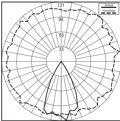
PRELIMINARY Candlepower trace of LED 60° flood canopy luminaire.
