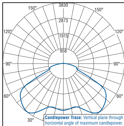
Independent Testing Laboratories certified test. Report No. ITL63657. Candlepower trace of 6000K, 120 LED sparkle petroleum area luminaire with 11,788 initial delivered lumens operating at 350mA. All published luminaire photometric testing performed to IESNA LM-79-08 standards.
