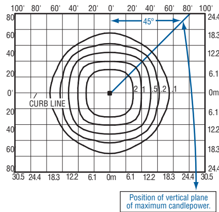
Isofootcandle plot of 6000K, 120 LED sparkle petroleum area luminaire at 25' A.F.G. Luminaire with 11,500 initial delivered lumens operating at 350mA. Initial FC at grade.
