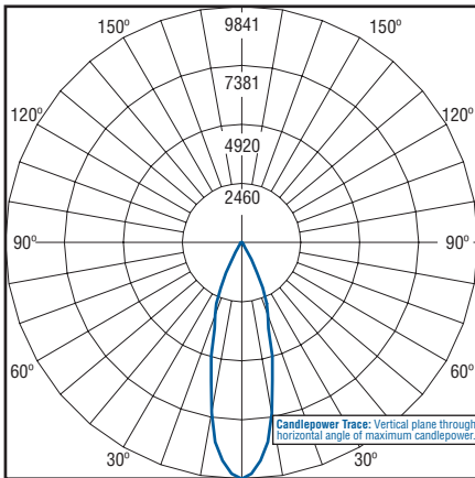
Preliminary candlepower trace of 4000K, 20 LED 25° flood luminaire with 11,148 initial delivered lumens operating at 700mA. Scaled from FLD-EDG-25-**-06-D-UL-7800-40K. All published luminaire photometric testing performed to IESNA LM-79-08 standards.
