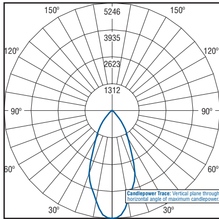
Preliminary candlegpower trace of 4000K, 20 LED 40° flood luminaire with 10,577 initial delivered lumens operating at 700mA. Scaled from FLD-EDG-40-**-06-D-UL-40K. All published luminaire photometric testing performed to IESNA LM-79-08 standards.
