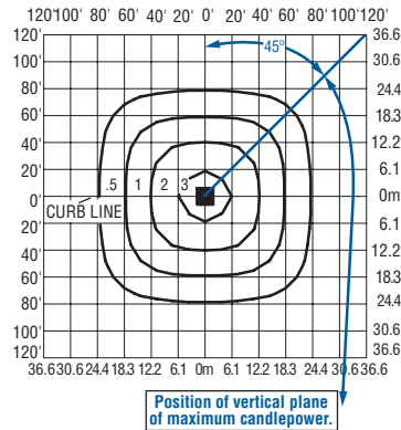
Isofootcandle plot of 6000K, 20 LED Petroleum symmetric parking structure luminaire at 15' (4.6m) A.F.G. Luminaire with 2,286 initial delivered lumens operating at 350mA. Initial FC at grade.
