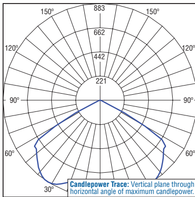
Candlepower trace of 6000K, 20 LED Petroleum Symmetric parking structure luminaire with 2,286 initial delivered lumens operating at 350mA. Configured from ITL66685, CAN-304-PS-**-06-D-UL-525. All published luminaire photometric testing performed to IESNA LM-79-08 standards.
