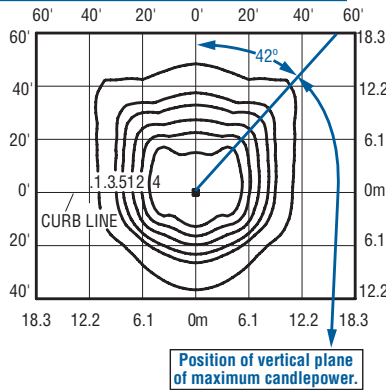
Position of vertical plane of maximum candlepower.
