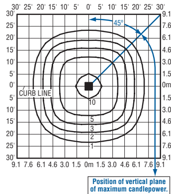
Isofootcandle plot of 5700K, 40 LED Type V Short 304 series soffit luminaire at 15' A.F.G. Luminaire with 4,202 initial delivered lumens operating at 700mA. Initial FC at grade.
