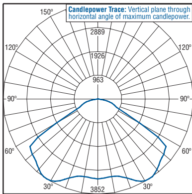
Independent Testing Laboratories certified test. Report No. ITL66685. Candlepower trace of 6000K, 60 LED Sparkle Petroleum Optic Scaled from CAN-304-SL-**-D-UL-700 with 11,973 initial delivered lumens operating at 700mA. All published luminaire photometric testing performed to IESNA LM-79-08 standards.
