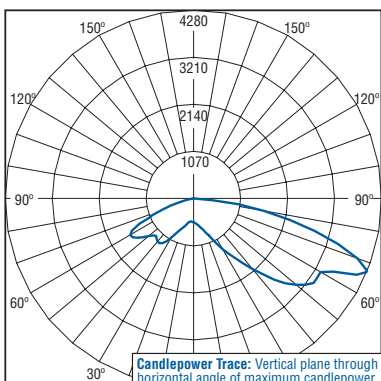
Independent Testing Laboratories certified test. Report No. ITL68432. Candlepower trace of 4300K, 40 LED LEDway Streetlight luminaire with IESNA Type II Medium distribution w/ partial backlight control. Luminaire with 5,725 initial delivered lumens operating at 700mA. All published luminaire photometric testing performed to IESNA LM-79-08 standards.
