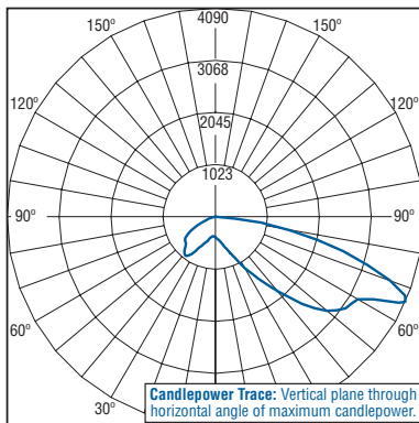
Independent Testing Laboratories certified test. Report No. ITL68358. Candlepower trace of 6000K, 40 LED LEDway Streetlight luminaire with IESNA Type II Medium distribution w/ backlight control. Luminaire with 5,373 initial delivered lumens operating at 700mA. All published luminaire photometric testing performed to IESNA LM-79-08 standards.
