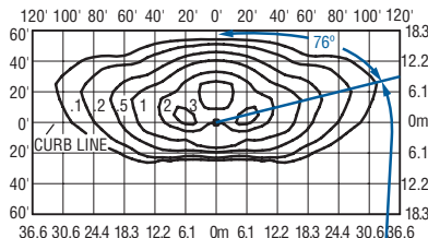
Isofootcandle plot of 6000K, 90 LED LEDway Streetlight luminaire with IESNA Type II Medium distribution w/ partial backlight control mounted at 25' A.F.G. Luminaire with 13,196 initial delivered lumens operating at 700mA. Initial FC at grade.
