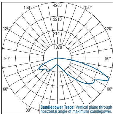
Independent Testing Laboratories certified test. Report No. ITL68432. Candlepower trace of 6000K, 40 LED LEDway Streetlight luminaire with IESNA Type II Medium distribution w/ partial backlight control. Luminaire with 5,725 initial delivered lumens operating at 700mA. All published luminaire photometric testing performed to IESNA LM-79-08 standards.
