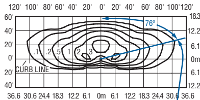
Isofootcandle plot of 6000K, 90 LED LEDway Streetlight luminaire with IESNA Type II Medium distribution w/ backlight control mounted at 25' A.F.G. Luminaire with 11,256 initial delivered lumens operating at 700mA. Initial FC at grade.
