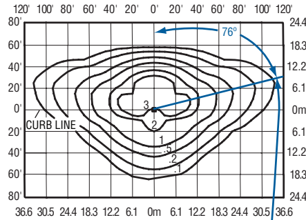
Position of vertical plane of maximum candlepower.
