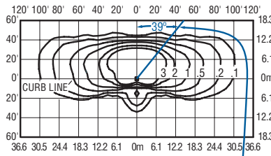
Position of vertical plane of maximum candlepower.
