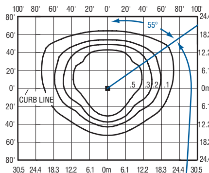
Position of vertical plane of maximum candlepower.
